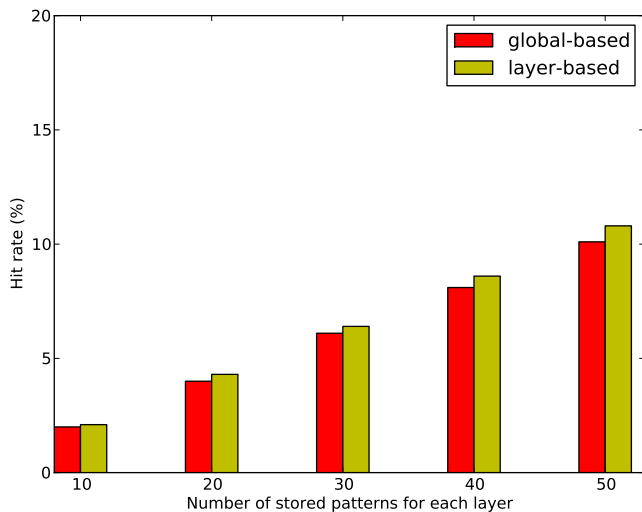
Fig. 3. The hit rate of exact pattern matching.
