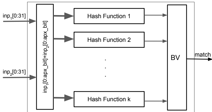
Fig. 5. The implementation of approximate pattern matching.
