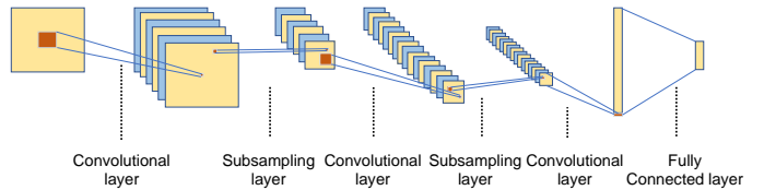
Fig. 2. An illustration of a convolutional neural network.
