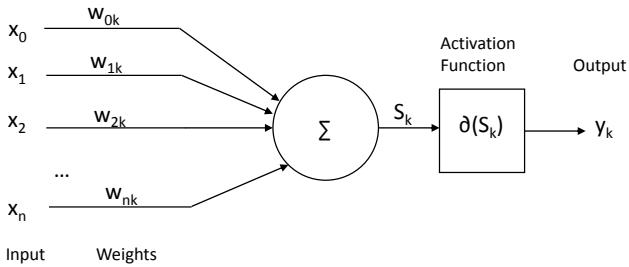
Fig. 1. The computation processes of an artificial neuron.
